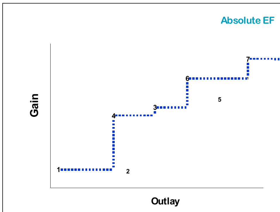
Figure 2-5 Absolute efficiency frontier given by the staircase incorporating an option (3) that is not clearly inefficient relative to the existing ones.
